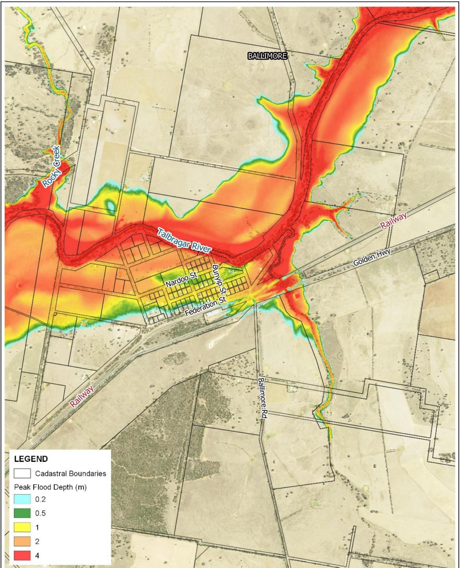
Title: Predicted Peak Flood Depths at Ballimore with Estimated 1955 Talbragar River Flows
