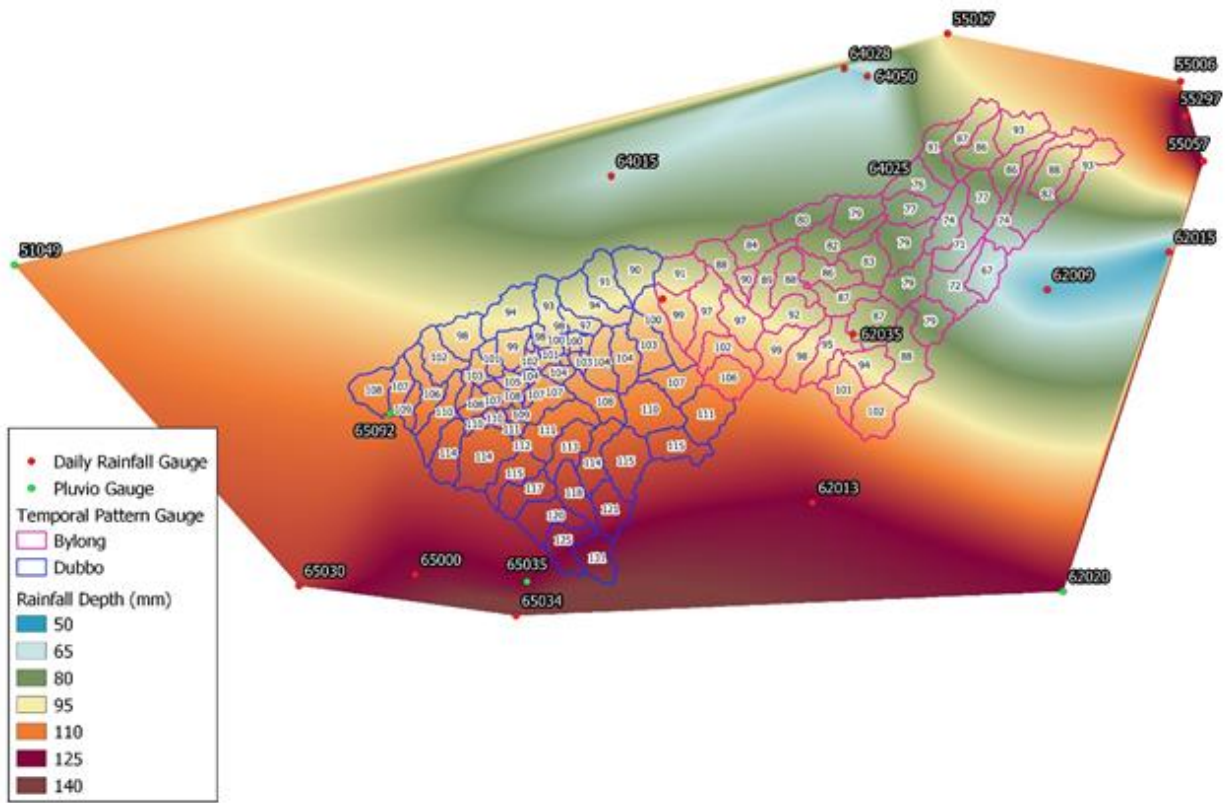
Figure 6.1 April 1990 Event Spatial Distribution of Rainfall Depth and Network of Gauges (120 hours to 9am 22 April)
