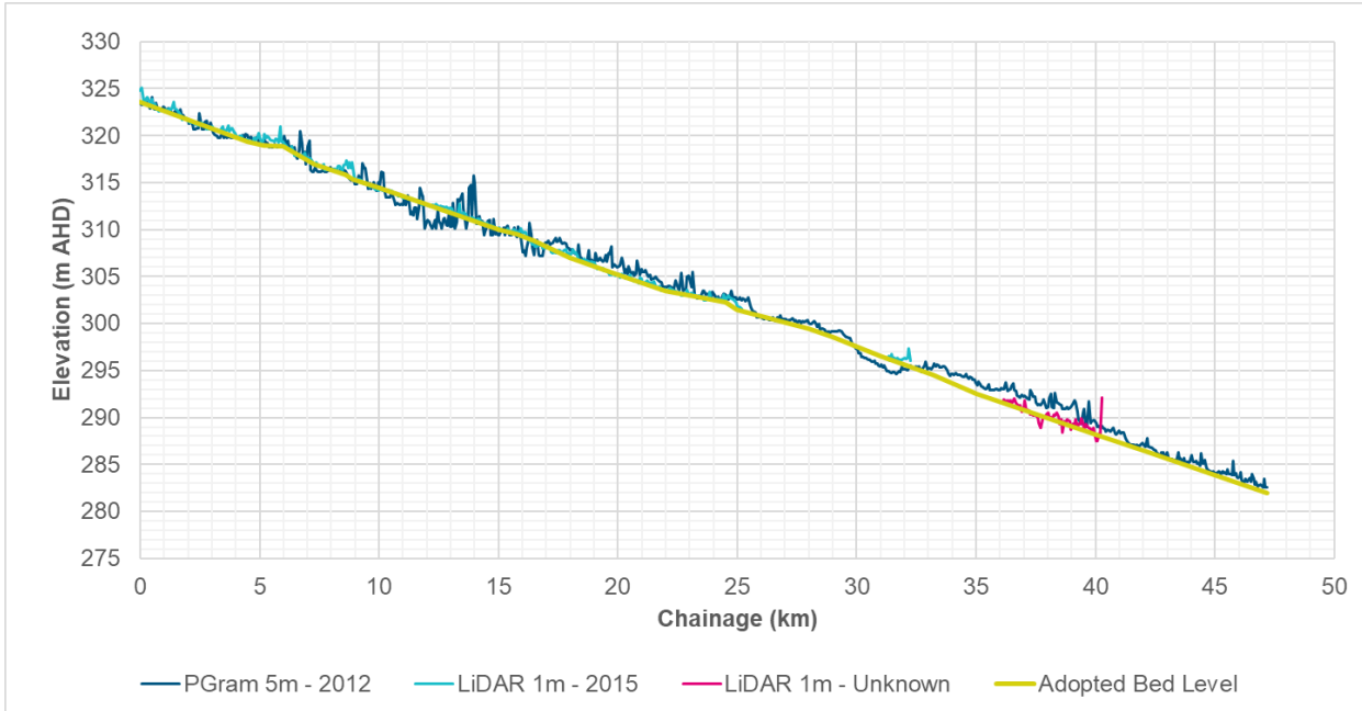
Figure 5.3 Adopted Talbragar River Channel Bed Invert Levels
