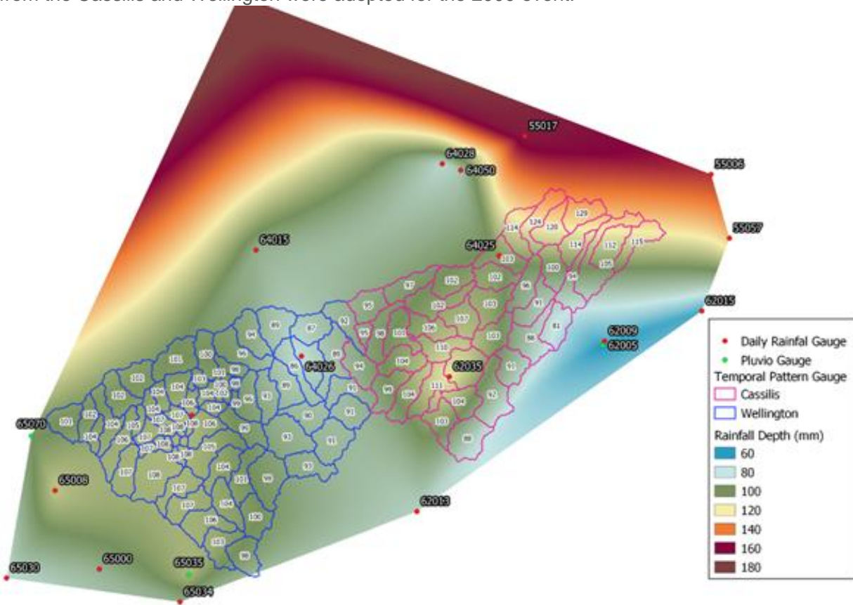
Figure 6.4 November 2000 Event Spatial Distribution of Rainfall Depth and Network of Gauges (96 hours to 9am 21 November)
